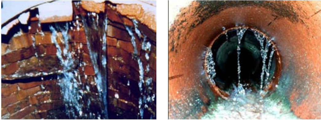
Storm water entering into the sewer system from a manhole, at left, and from a defect inside a pipe, at right.
